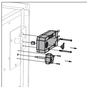
Type BFN(T) on CR2/CU2/ CU4/CU2-15:
