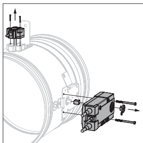
Type BFN(T) (-SR) on CR60/ CR120/CRS60/CU-LT(1s):
